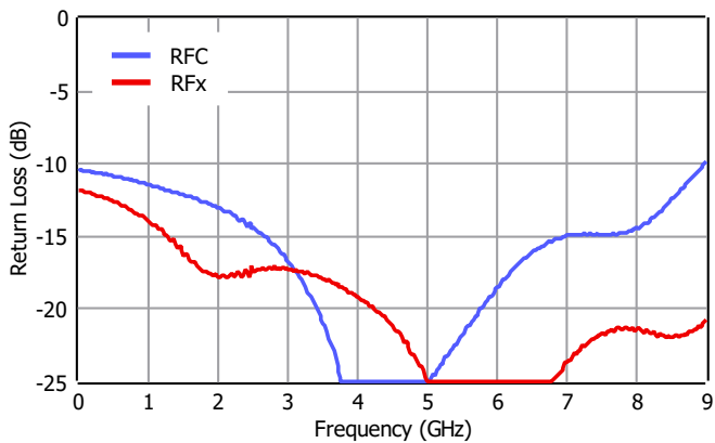
Return Loss
