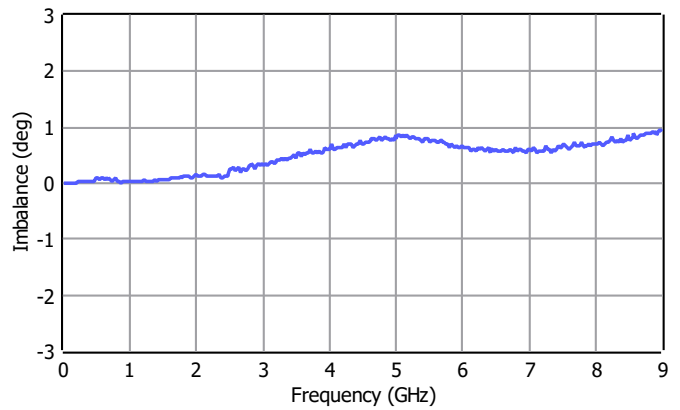
Phase Imbalance
