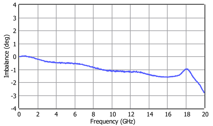
Phase Imbalance
