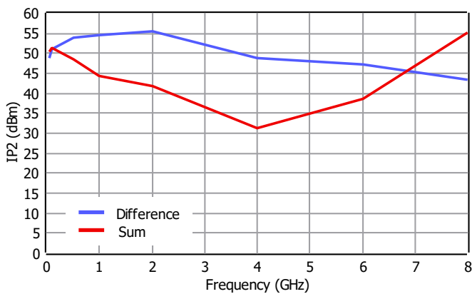
IP2 at Pout = 6dBm/tone
